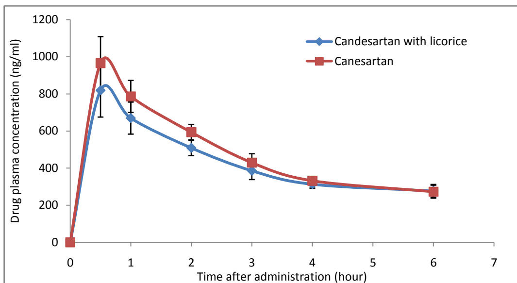
Figure 12: Rat plasma profile showing the changes in mean serum candesartan concentration with time after drug administration, comparing candesartan with liquorice juice and solitary drug use, each data point represents the mean \pm SEM (n=6).
