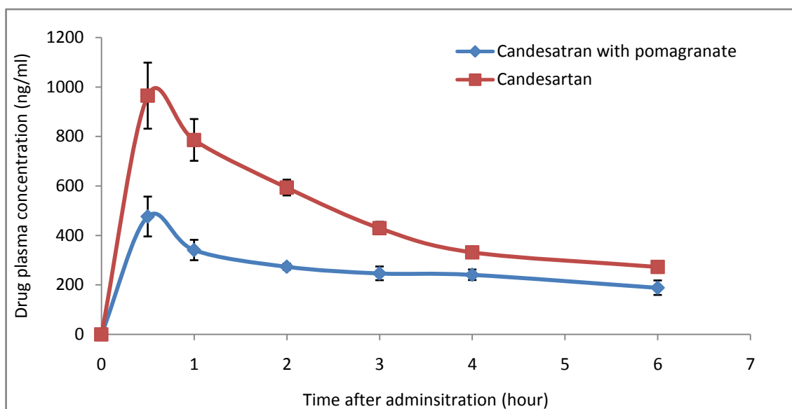
Figure 13: Rat plasma profile showing the changes in mean serum candesartan concentration with time after drug administration, comparing candesartan with pomegranate juice and solitary drug use, each data point represents the mean \pm SEM (n=3).
